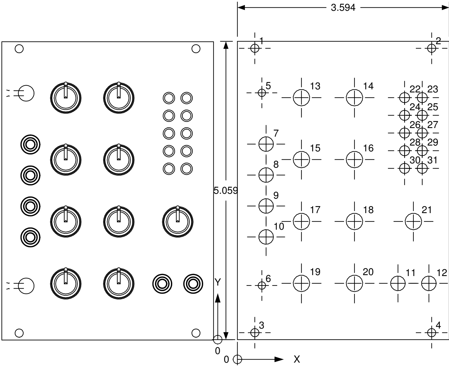
D102 OUTPUT MIXER PANEL LAYOUT
