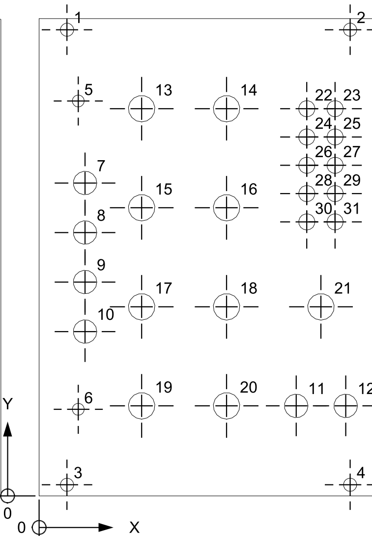
D102 OUTPUT MIXER PANEL LAYOUT
