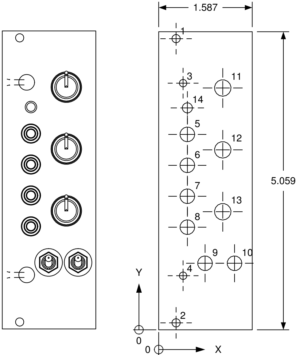
D103 REVERB DELAY PANEL LAYOUT
