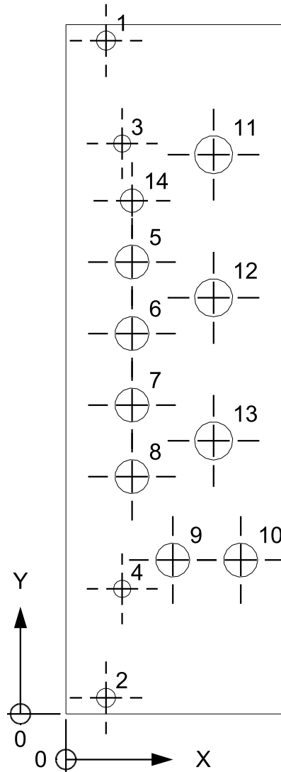
D103 REVERB DELAY PANEL LAYOUT
