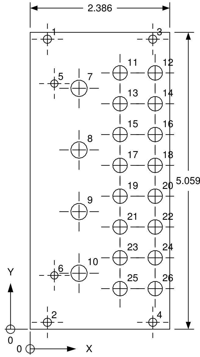
D105 QUAD CV PROC PANEL LAYOUT
