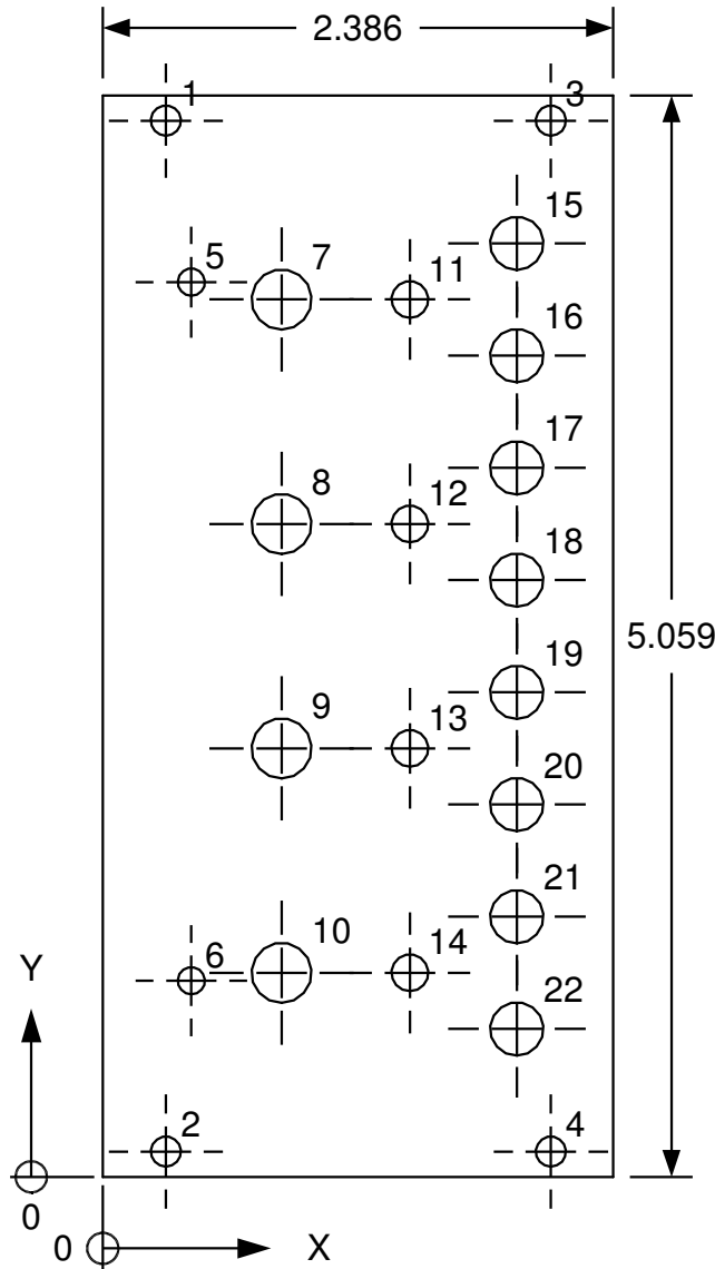
D106 STEP SEQUENCER PANEL LAYOUT
