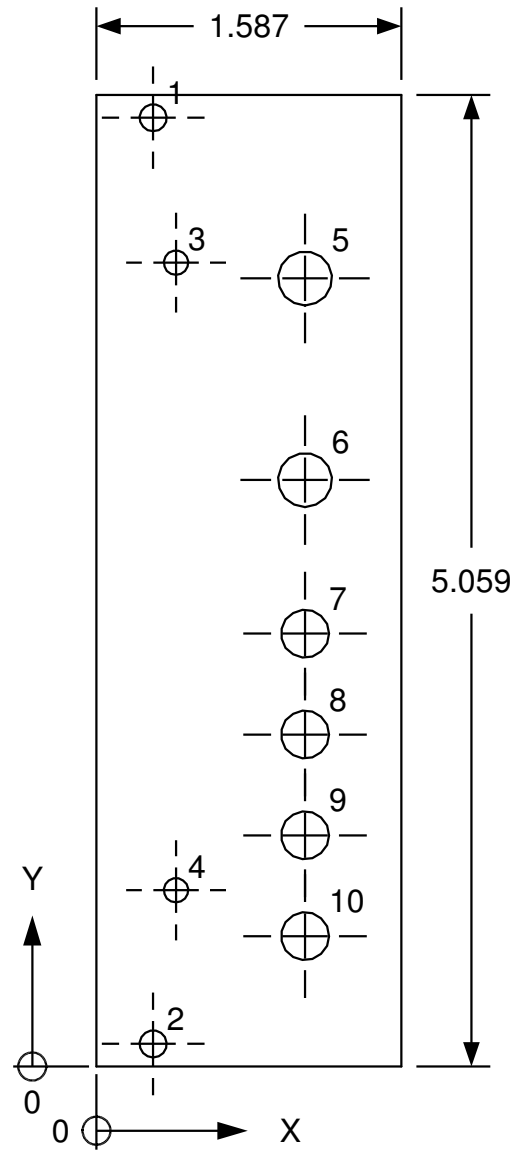
D107 DUAL SLEW PANEL LAYOUT
