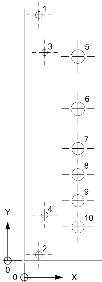
D107 DUAL SLEW PANEL LAYOUT
